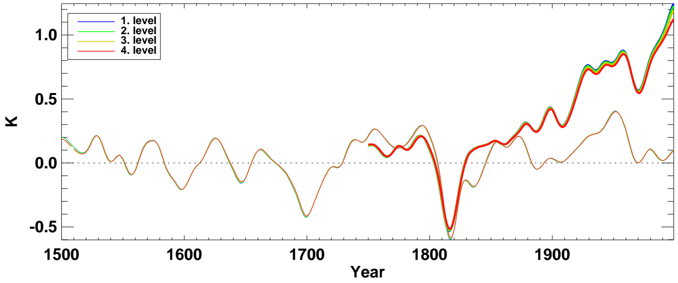
soilt from hadcm3 averaged over Tropics land (all levels)
