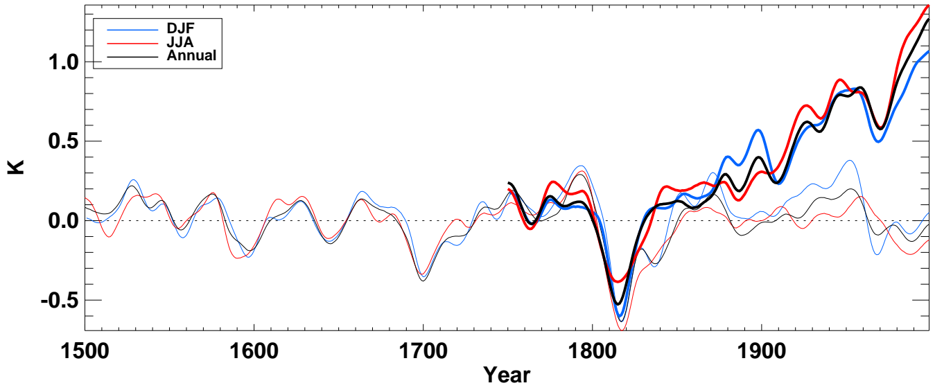
soilt from hadcm3 averaged over SH land (level 1. level only)
