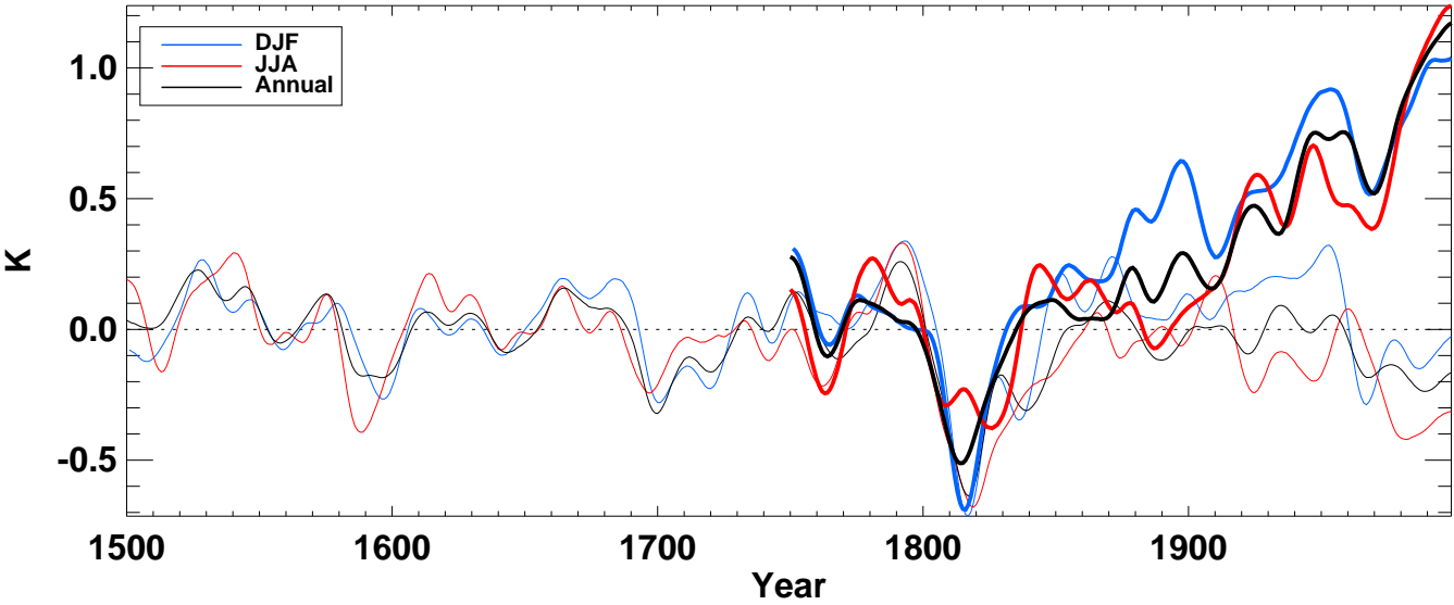
soilt from hadcm3 averaged over S-extratropics land (level 1. level only)
