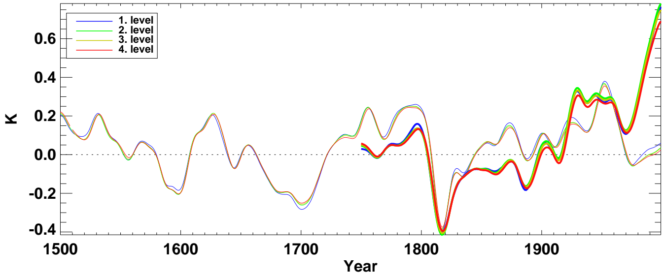
soilt from hadcm3 averaged over NH land (all levels)
