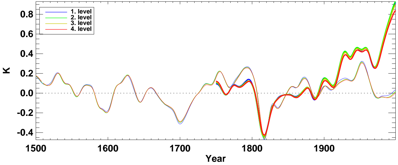
soilt from hadcm3 averaged over Global land (all levels)
