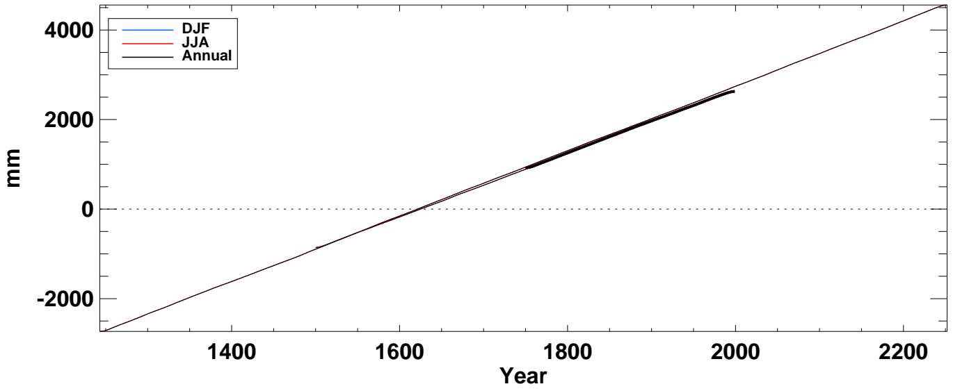
snowd from hadcm3 averaged over N-extratropics land
