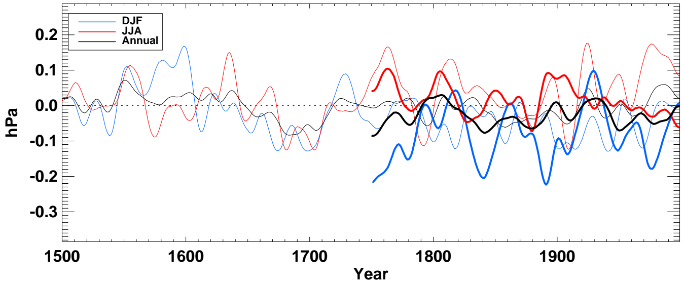
slp__ from hadcm3 averaged over Tropics ocean
