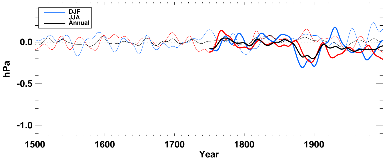
slp__ from hadcm3 averaged over SH ocean
