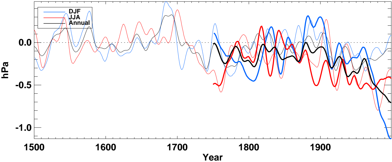
slp__ from hadcm3 averaged over SH land
