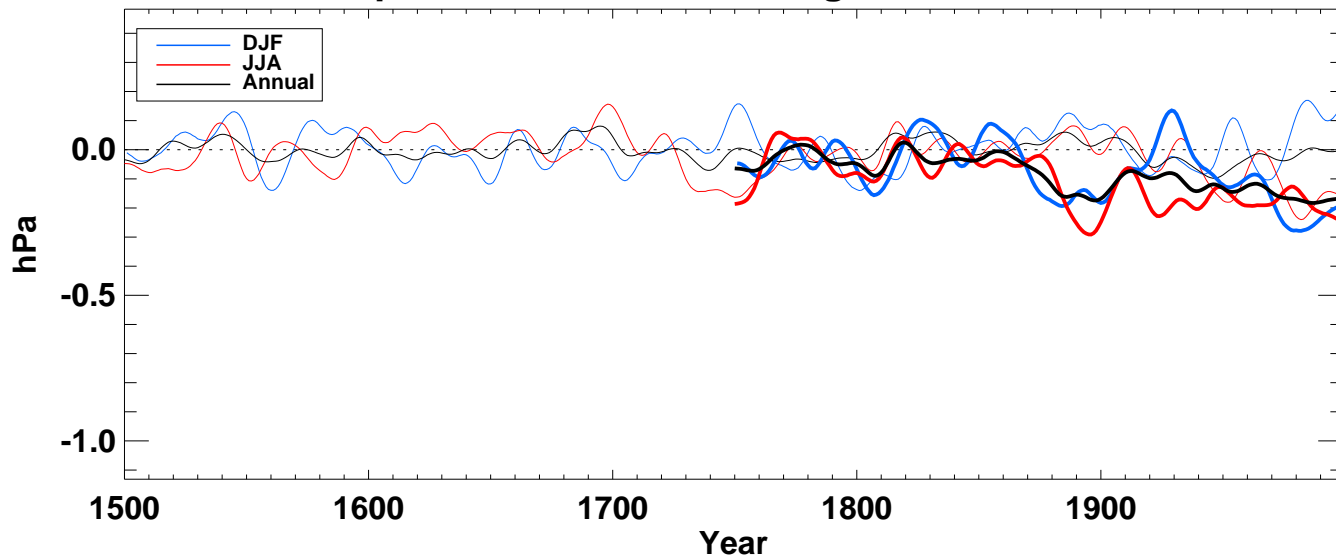
slp__ from hadcm3 averaged over SH full
