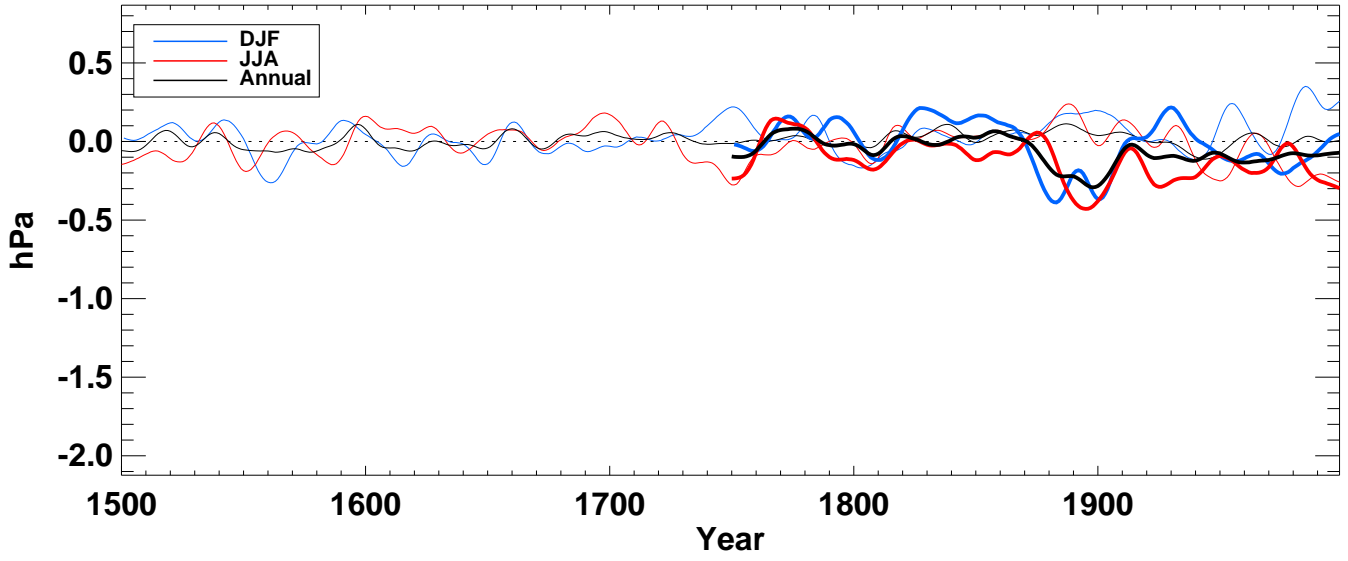
slp__ from hadcm3 averaged over S-extratropics ocean
