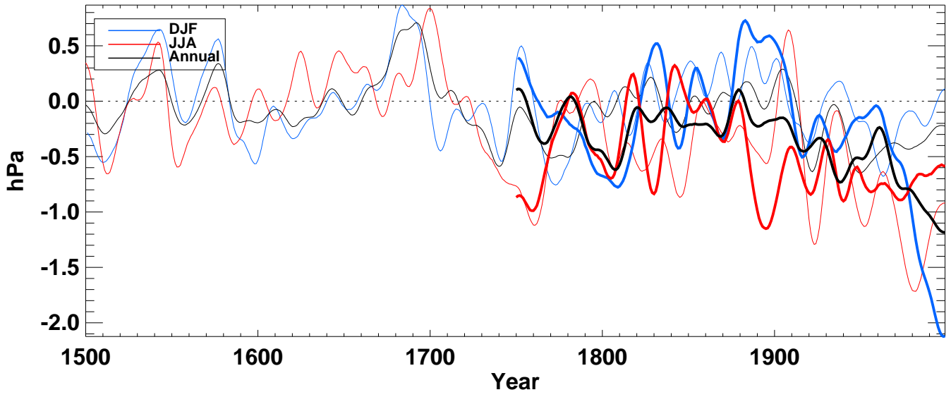
slp__ from hadcm3 averaged over S-extratropics land
