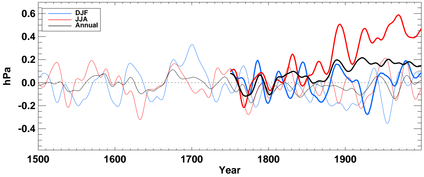
slp__ from hadcm3 averaged over N-extratropics land
