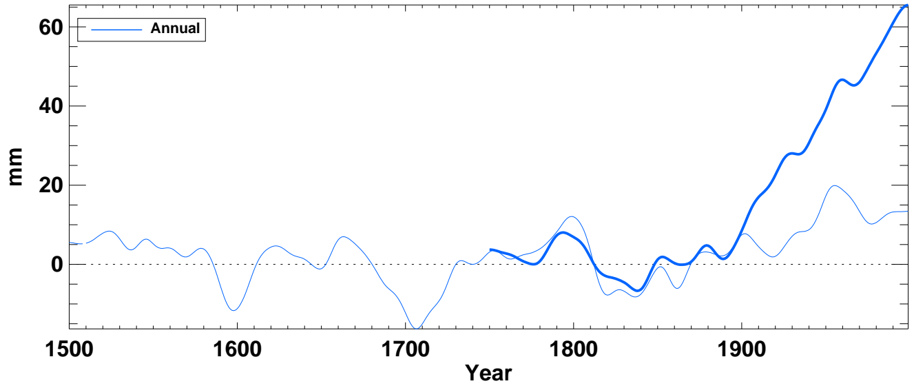
sealy from hadcm3 averaged over Tropics ocean
