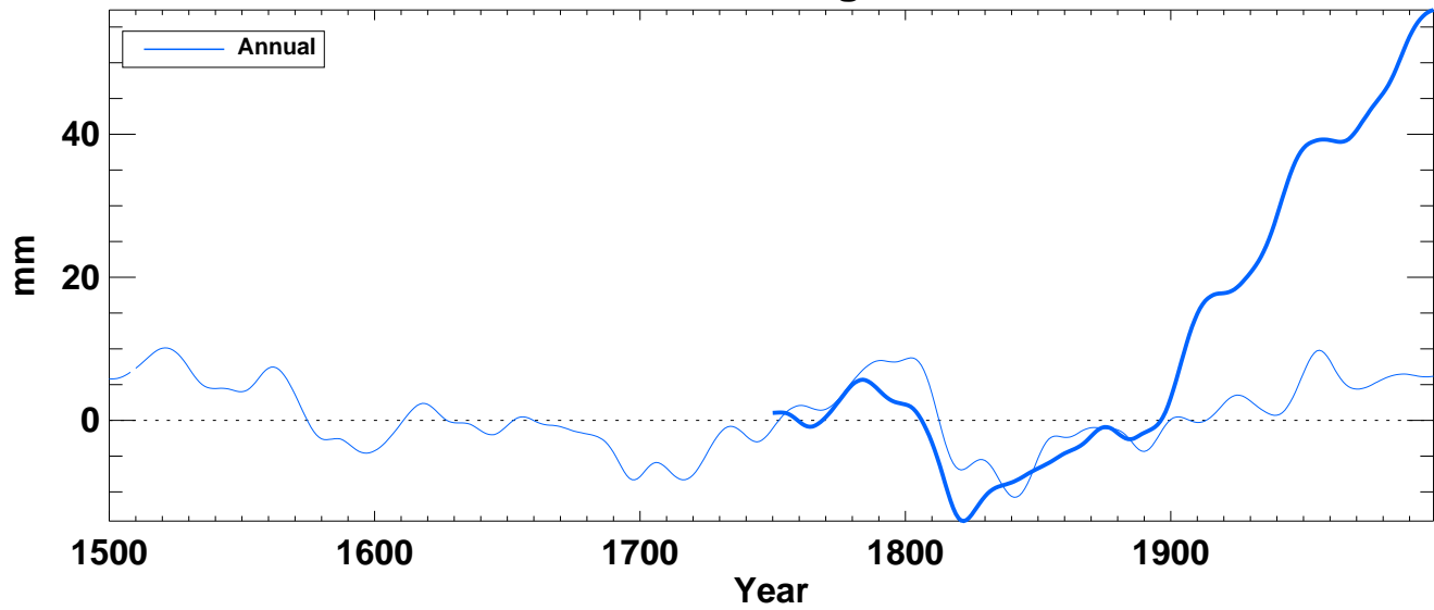
sealv from hadcm3 averaged over SH ocean
