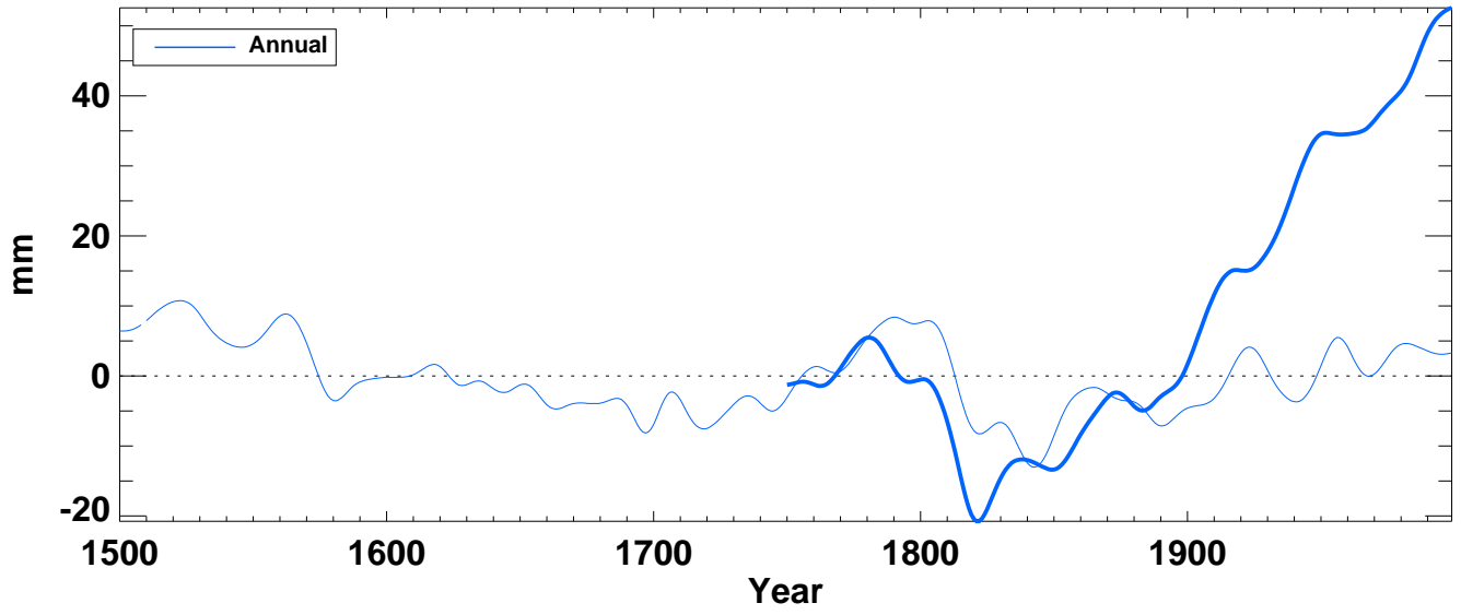
sealy from hadcm3 averaged over S-extratropics ocean
