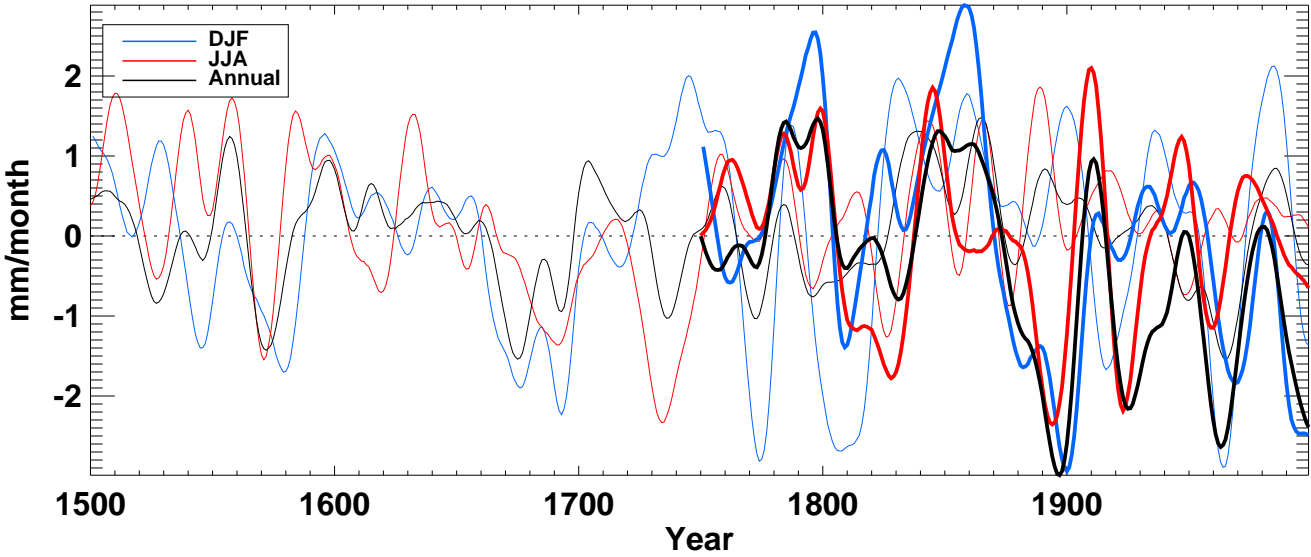
precip from hadcm3 averaged over Tropics land
