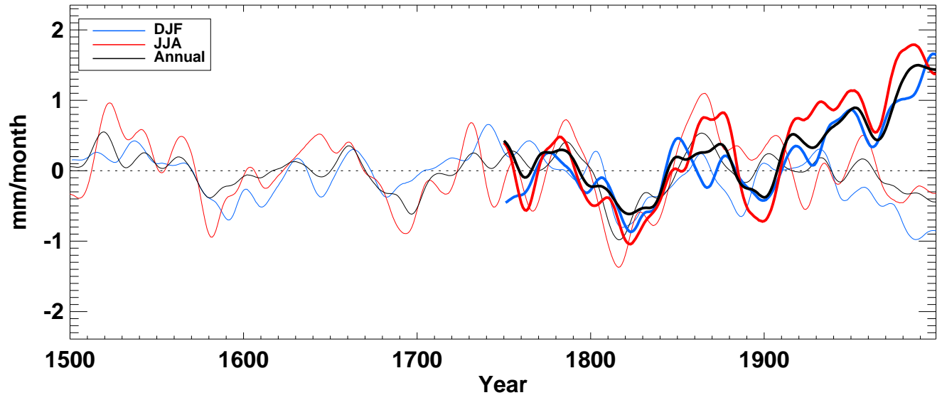
precip from hadcm3 averaged over S-extratropics ocean
