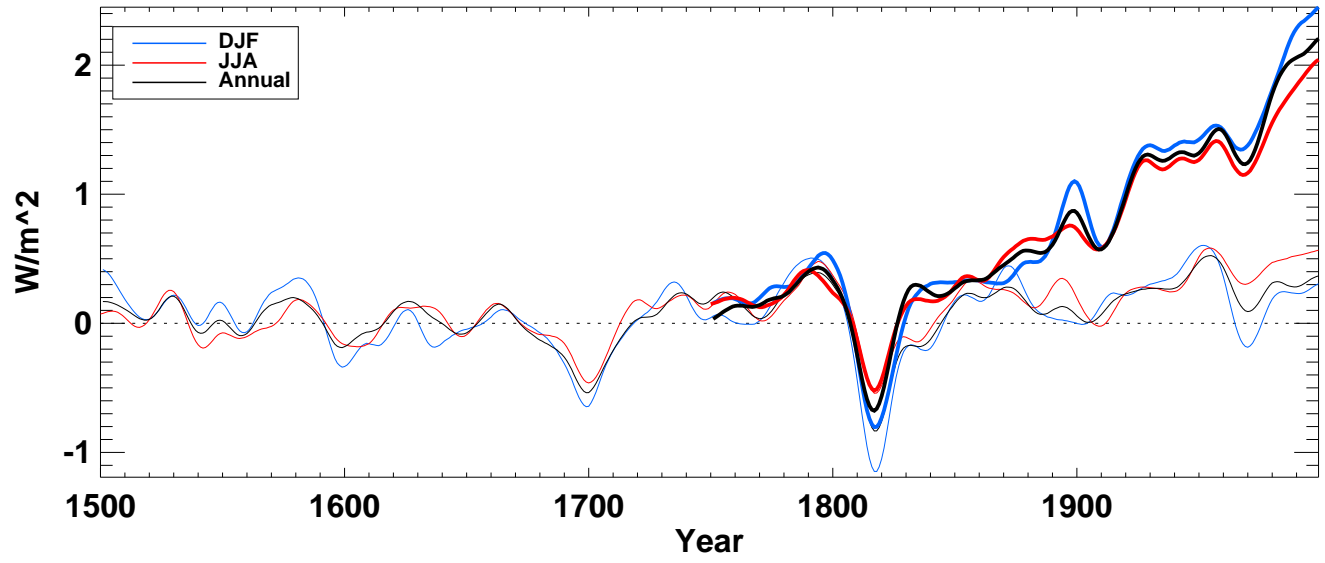
lwrad from hadcm3 averaged over SH ocean
