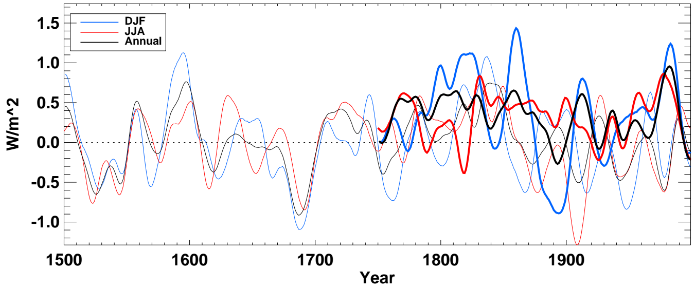
lwrad from hadcm3 averaged over S-extratropics land
