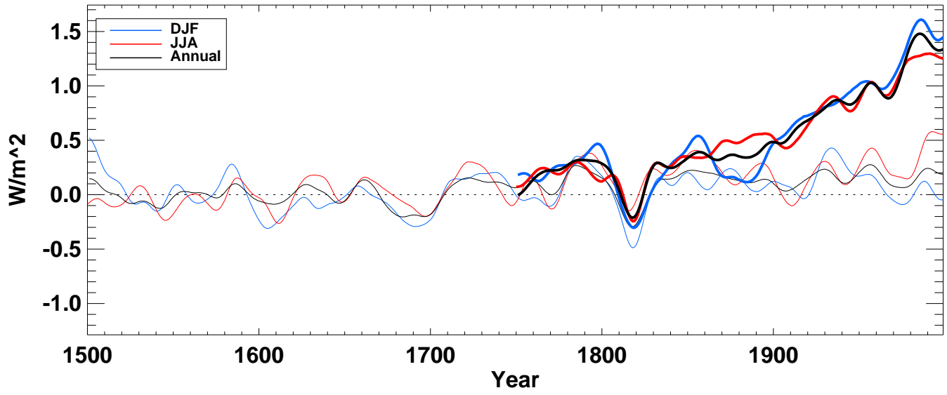
lwrad from hadcm3 averaged over S-extratropics full
