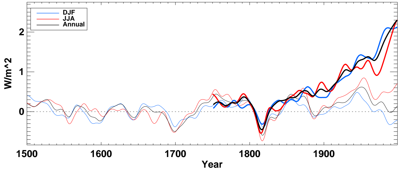
lwrad from hadcm3 averaged over NH ocean
