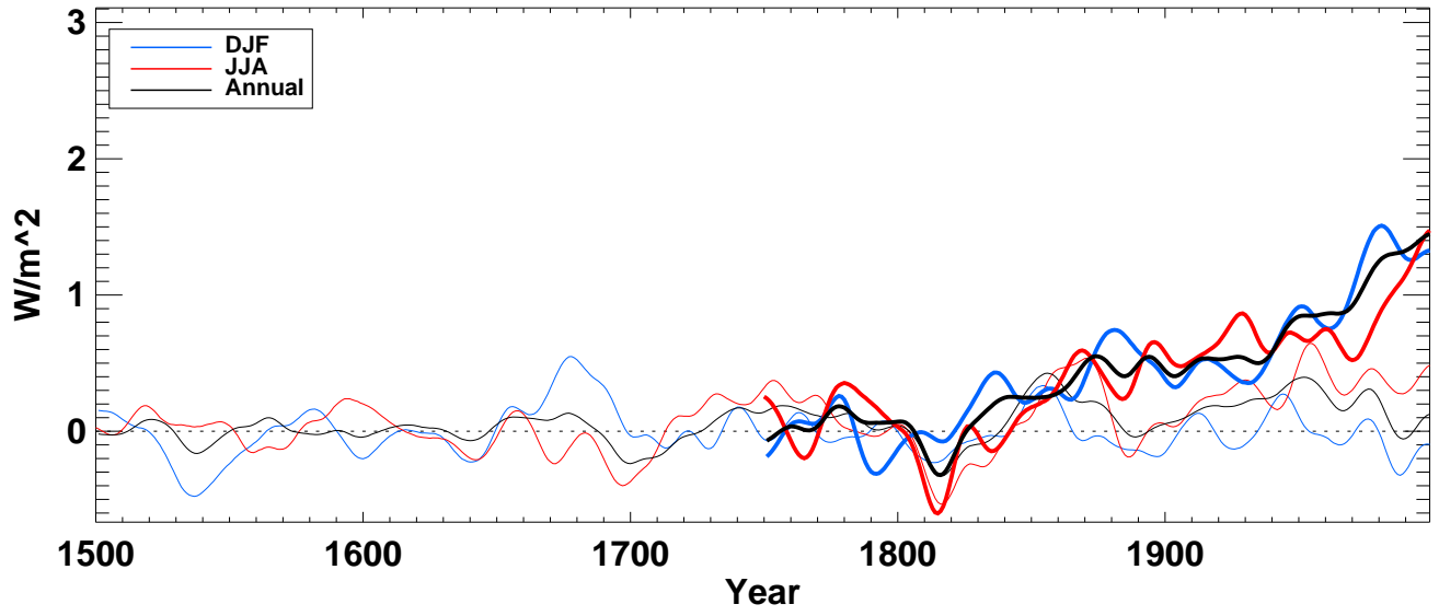
lwrad from hadcm3 averaged over N-extratropics ocean
