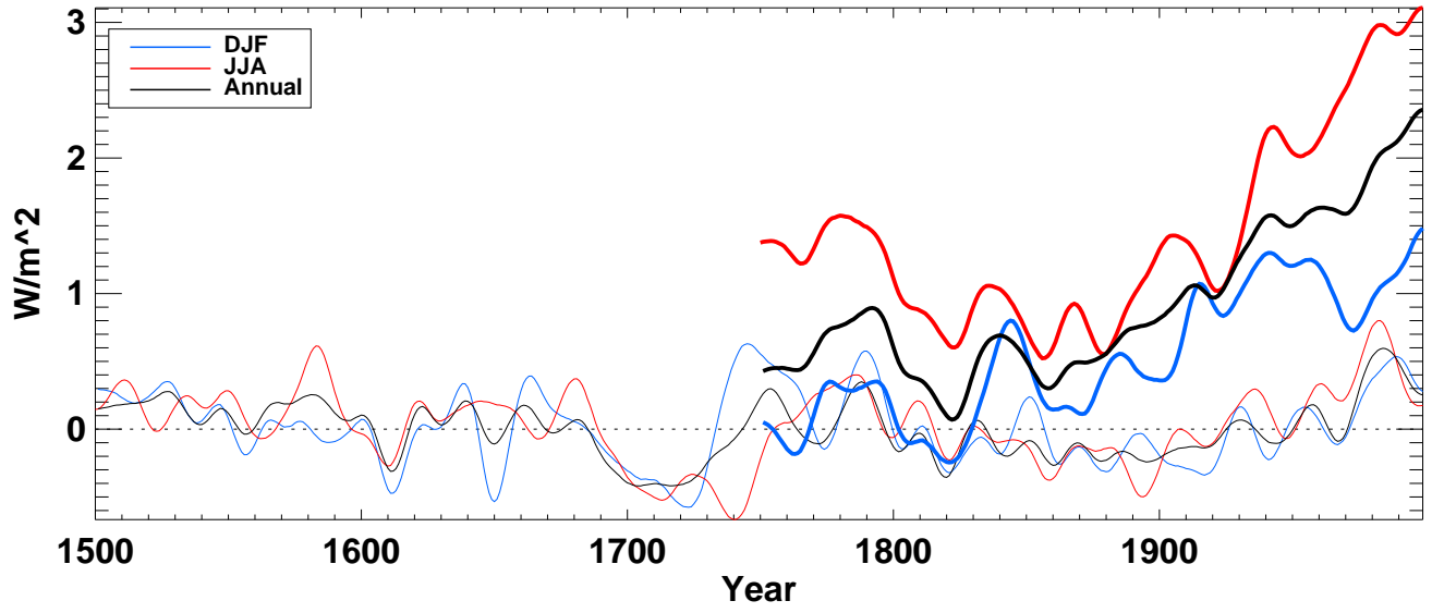
lwrad from hadcm3 averaged over N-extratropics land
