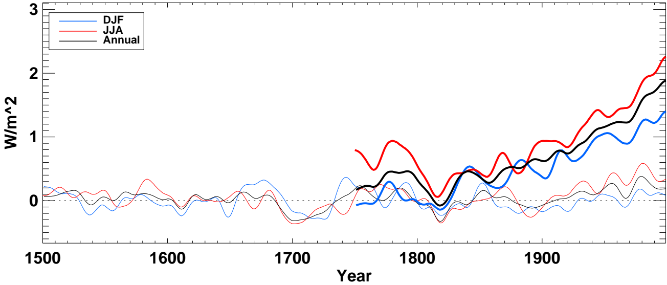
lwrad from hadcm3 averaged over N-extratropics full
