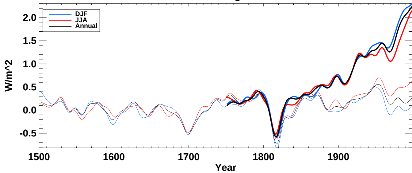
lwrad from hadcm3 averaged over Global ocean
