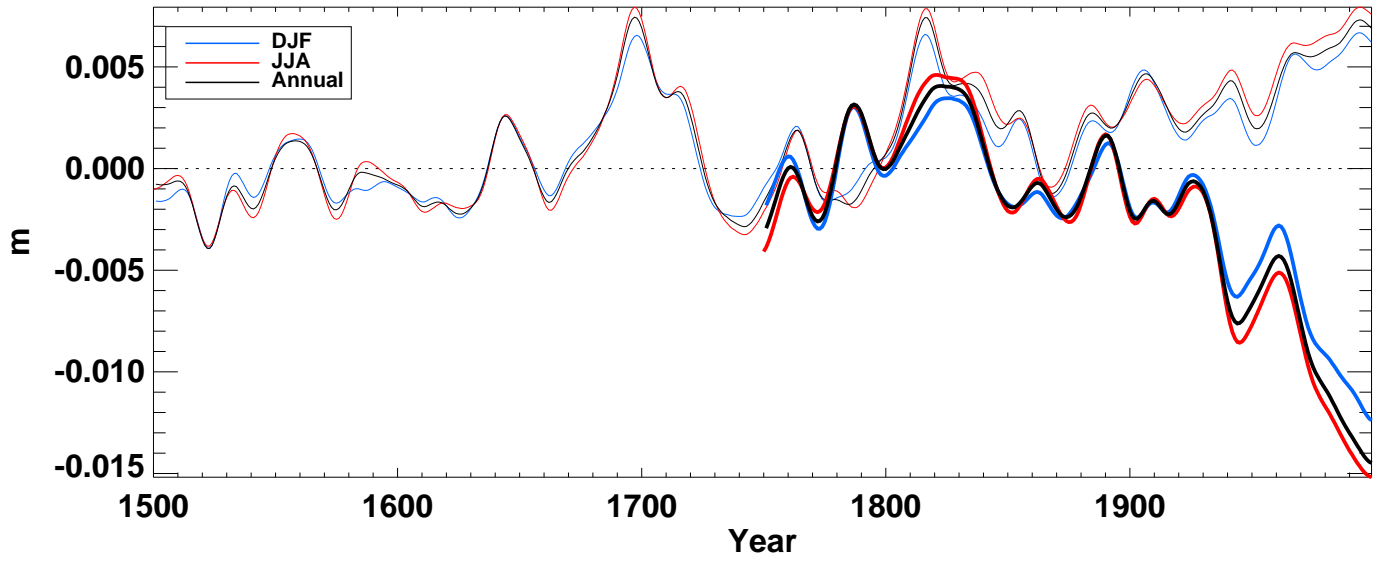
iceth from hadcm3 averaged over SH ocean
