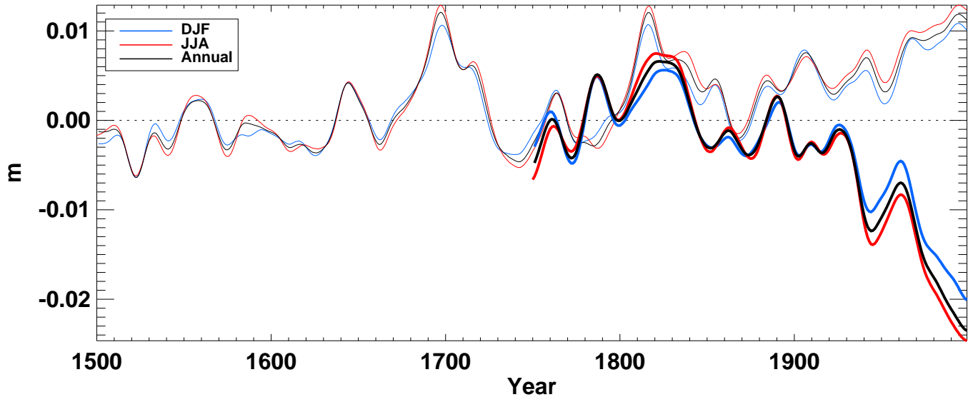
iceth from hadcm3 averaged over S-extratropics ocean
