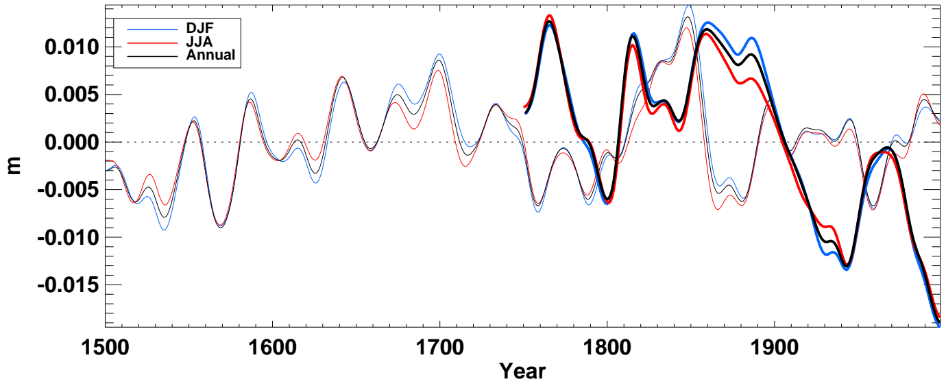
iceth from hadcm3 averaged over NH ocean
