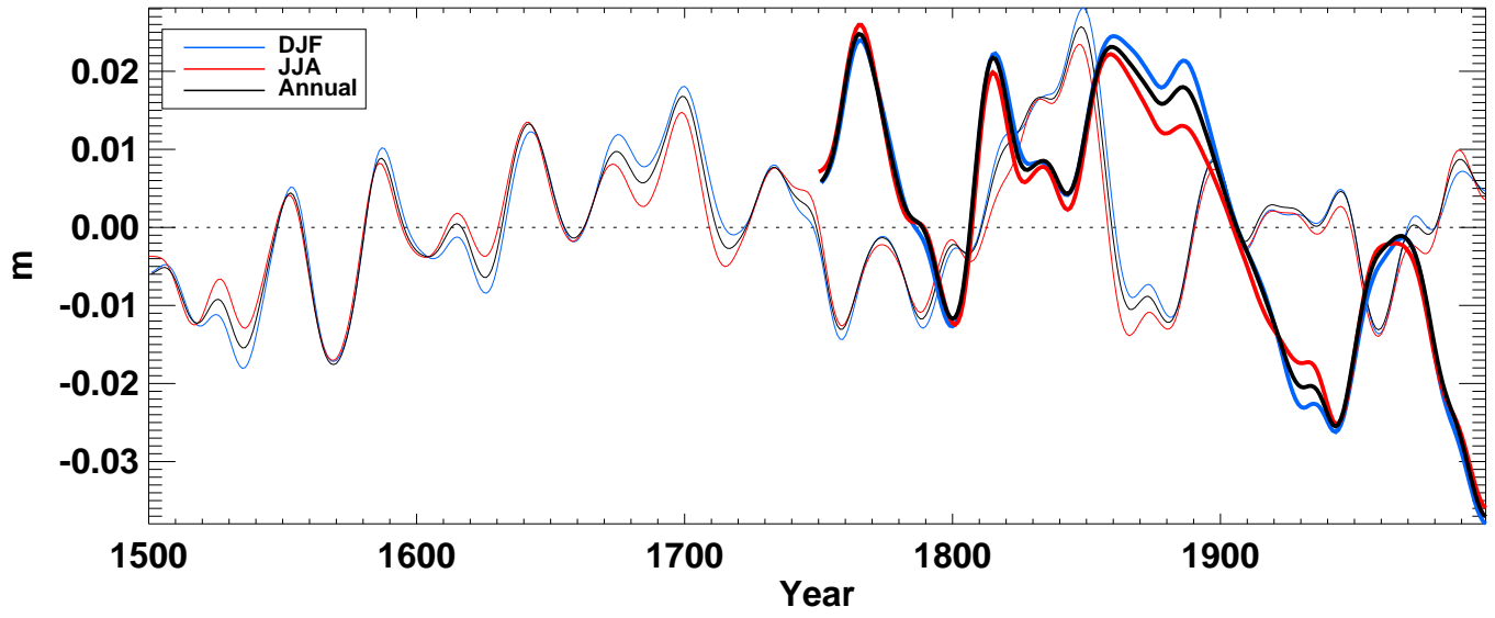
iceth from hadcm3 averaged over N-extratropics ocean
