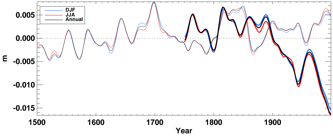
iceth from hadcm3 averaged over Global ocean
