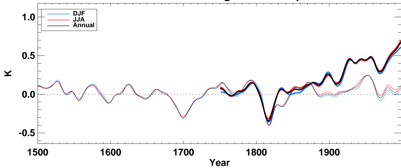
airtm from hadcm3 averaged over Tropics ocean
