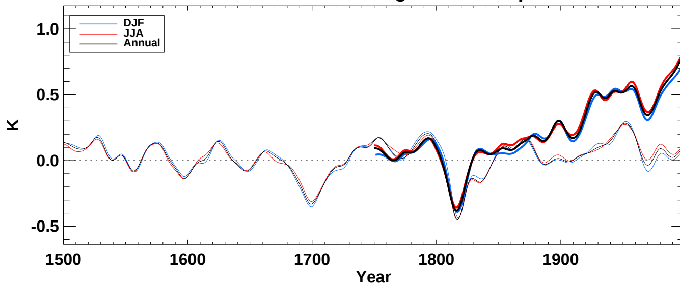
airtm from hadcm3 averaged over Tropics full
