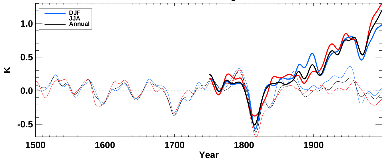
airtm from hadcm3 averaged over SH land
