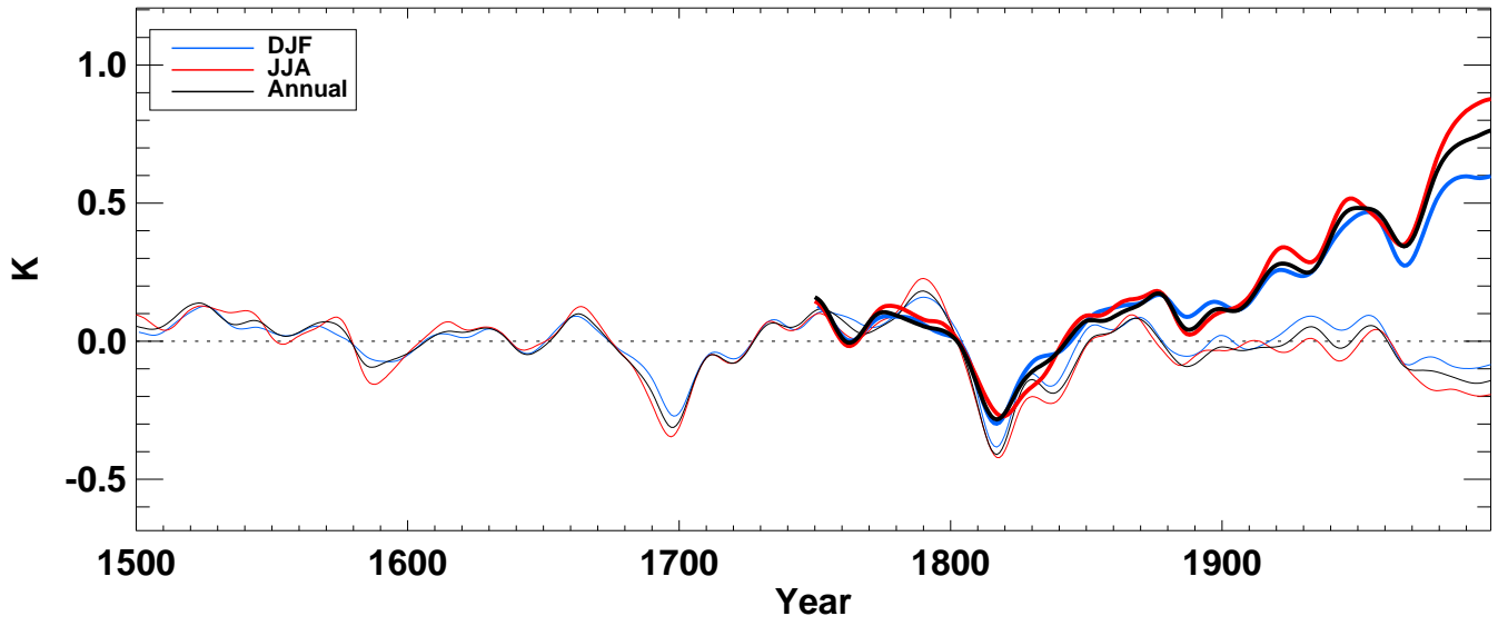
airtm from hadcm3 averaged over S-extratropics full
