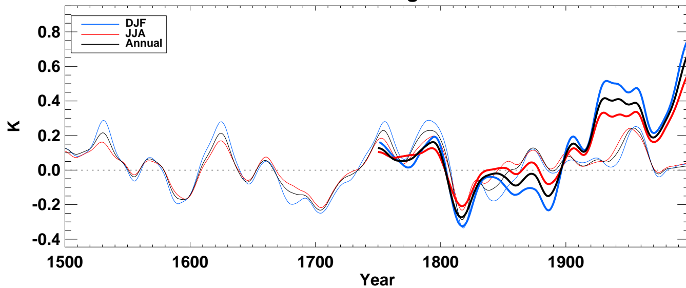
airtm from hadcm3 averaged over NH ocean
