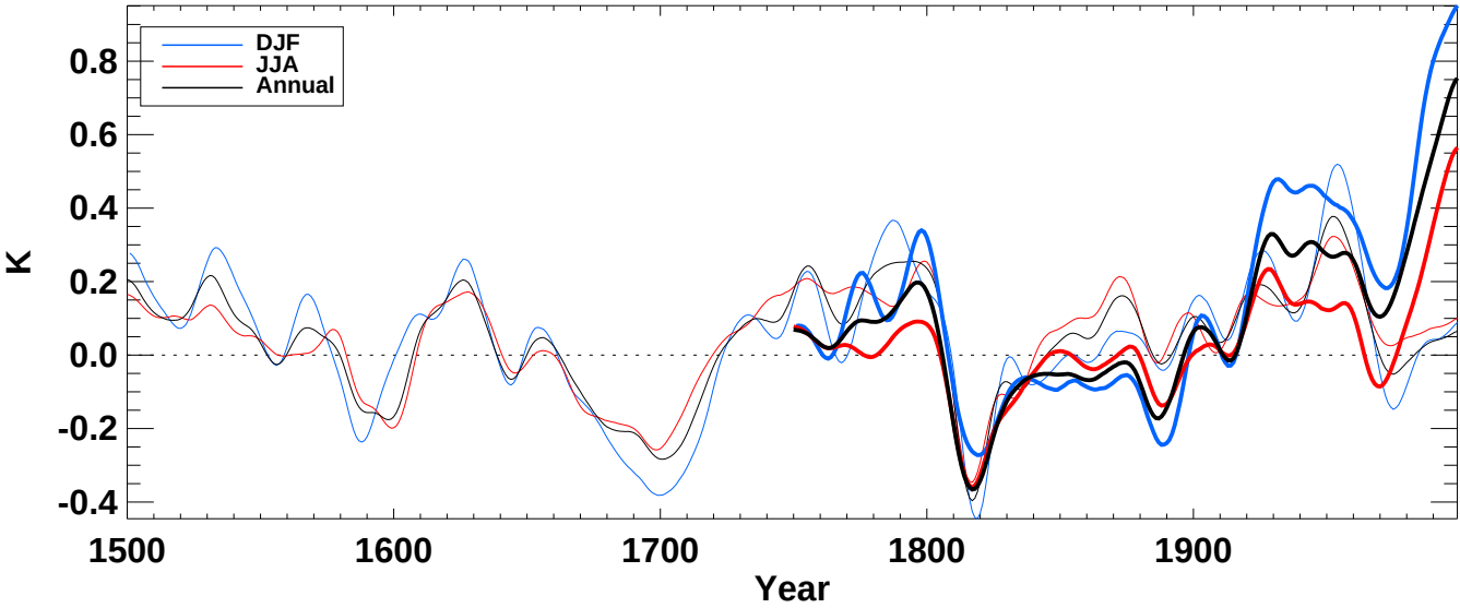
airtm from hadcm3 averaged over NH land
