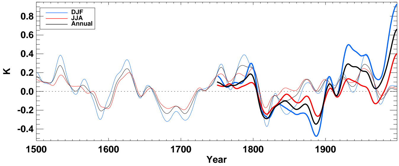
airtm from hadcm3 averaged over N-extratropics full
