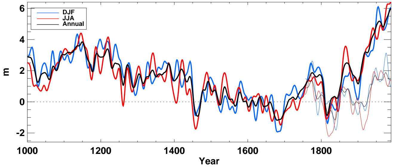
z850_ from echo-g averaged over Tropics ocean
