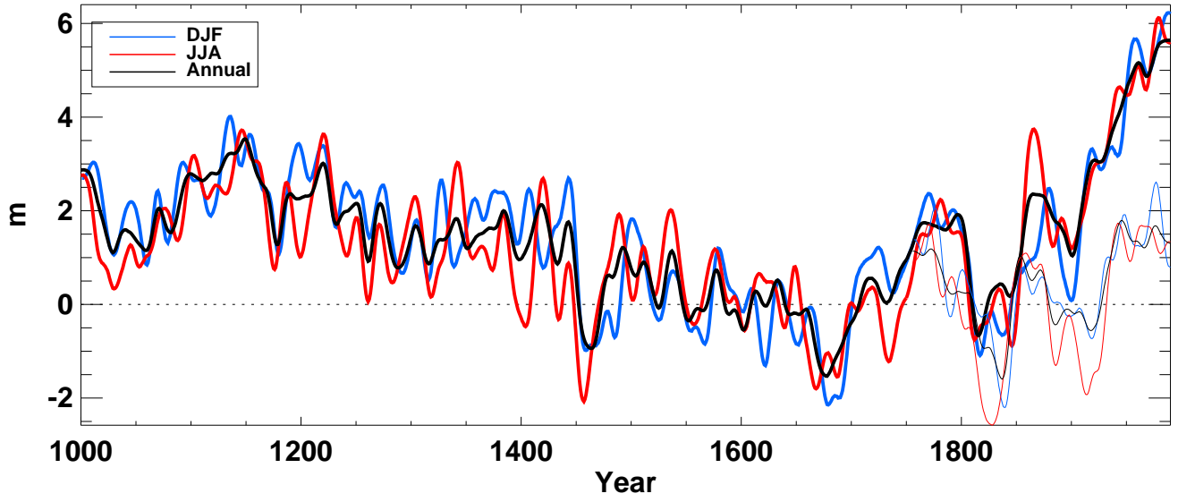
z850_ from echo-g averaged over Tropics land
