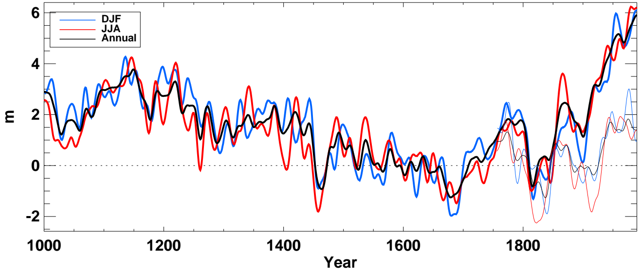
z850_ from echo-g averaged over Tropics full
