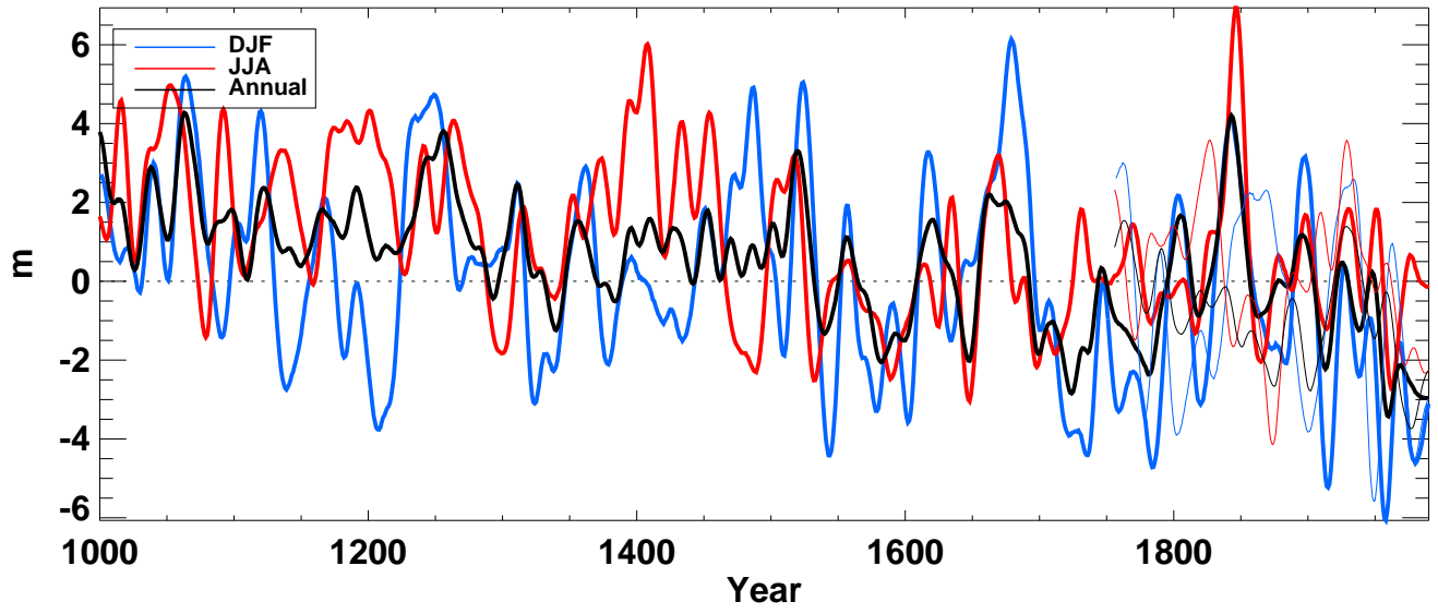
z850_ from echo-g averaged over SH land
