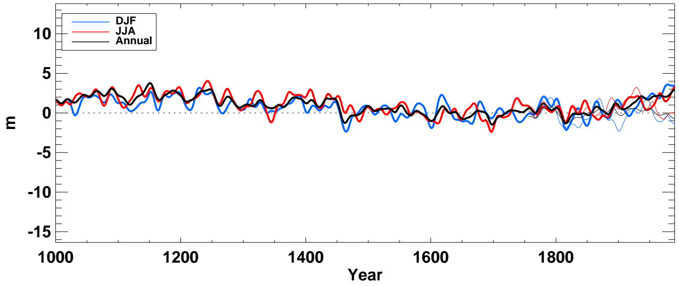
z850_ from echo-g averaged over S-extratropics ocean
