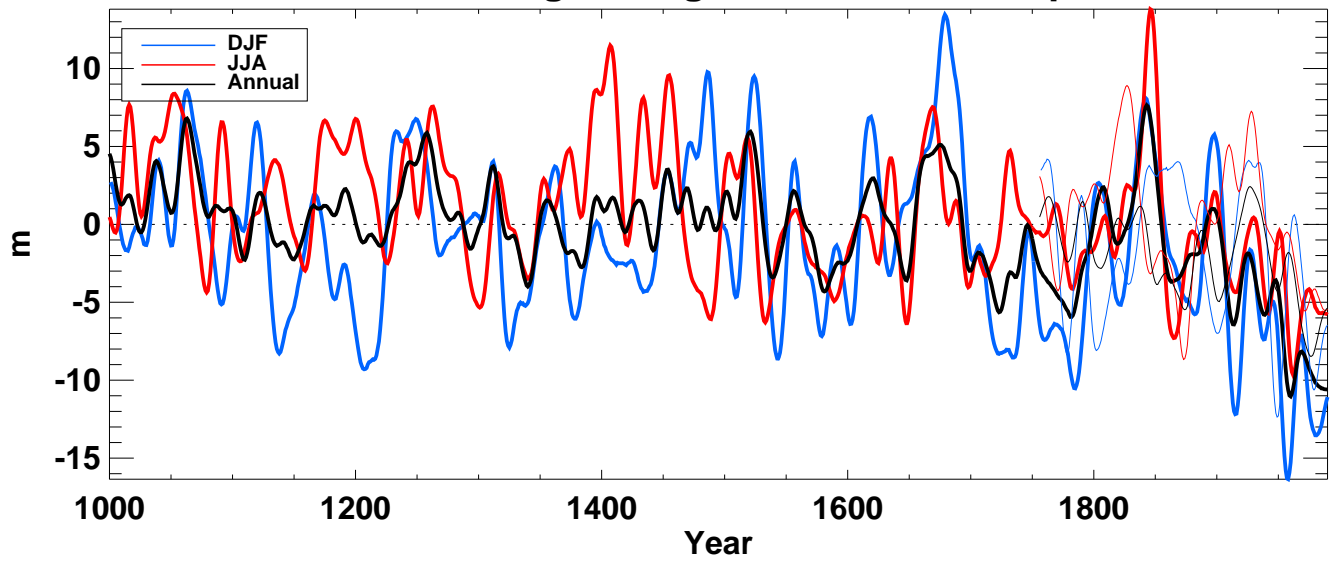
z850_ from echo-g averaged over S-extratropics land
