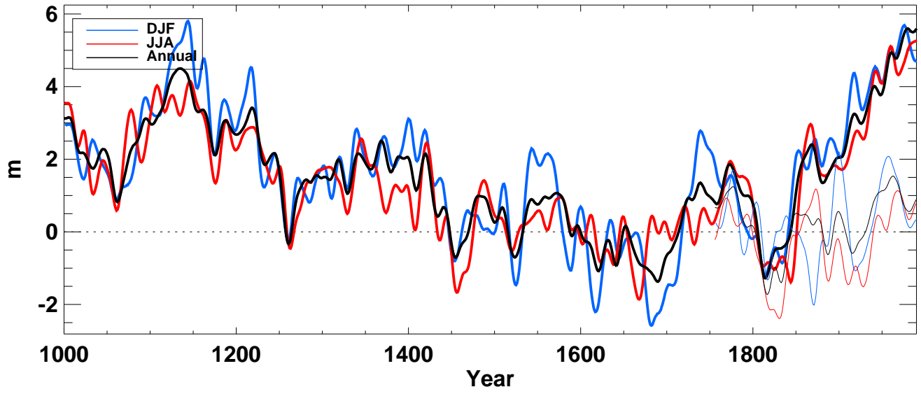
z850_ from echo-g averaged over NH ocean
