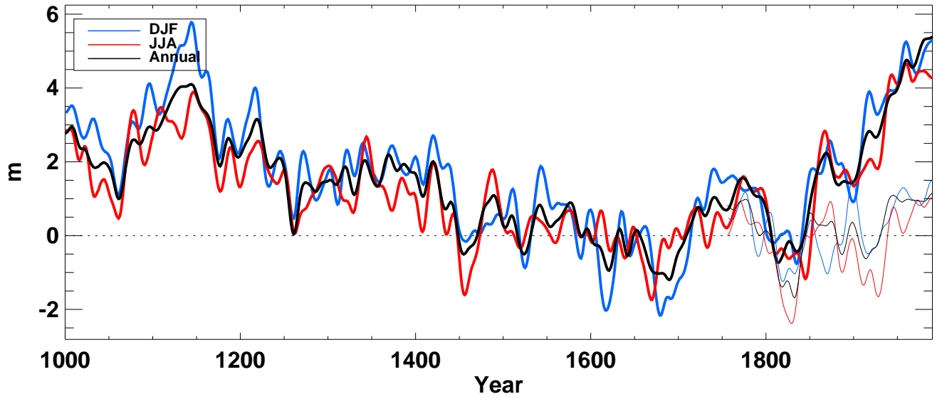
z850_ from echo-g averaged over NH full
