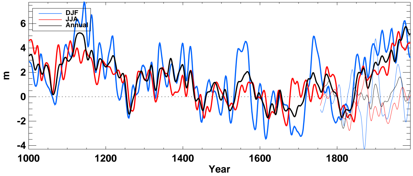
z850_ from echo-g averaged over N-extratropics ocean
