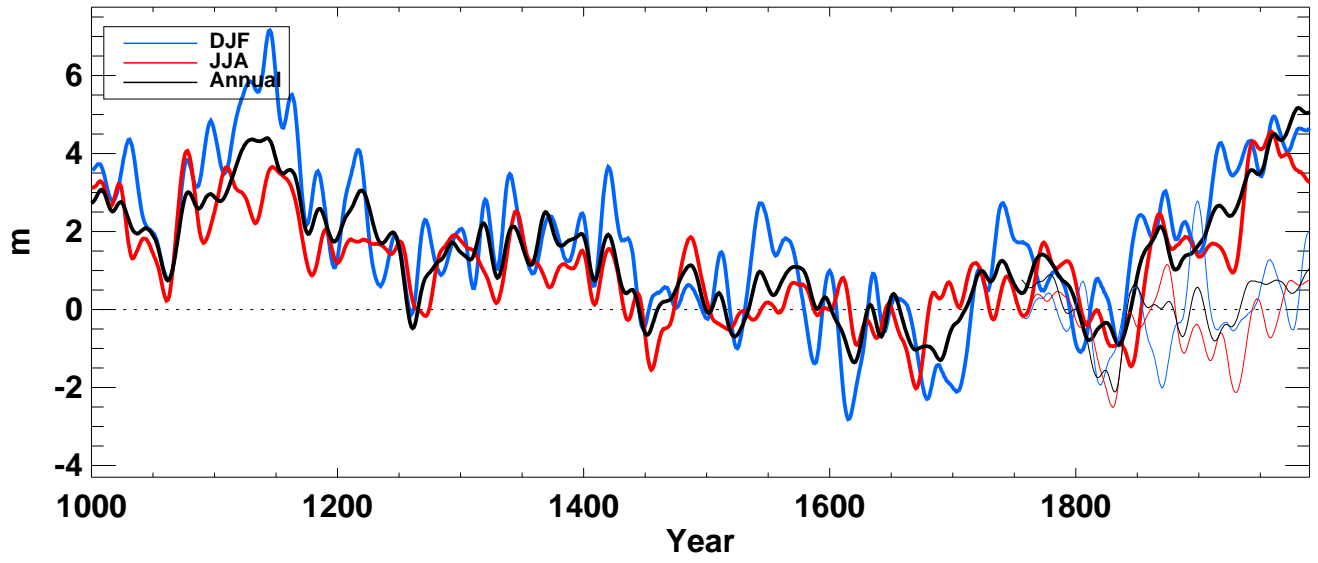
z850_ from echo-g averaged over N-extratropics full
