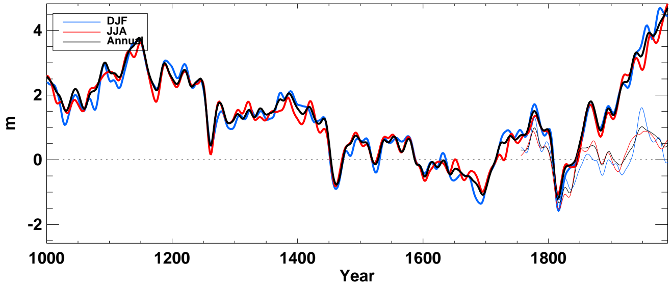
z850_ from echo-g averaged over Global ocean
