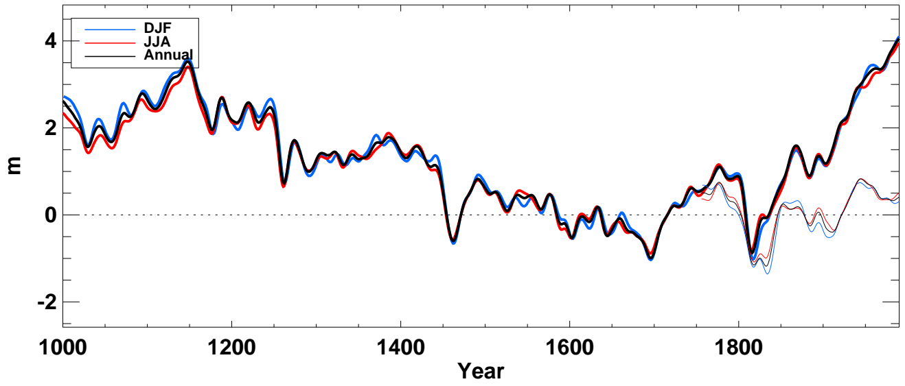
z850_ from echo-g averaged over Global full
